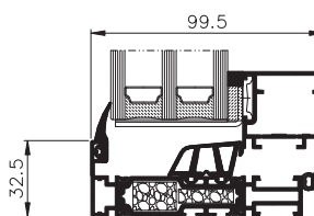
opening window – cross section
